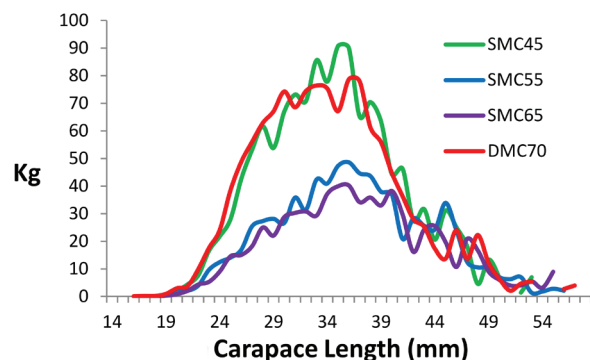
Figure 3. Plot of total raised weights of Nephrops per Carapace Length from four test gears: DMC70 = diamond mesh cod-end with 70 mm nominal mesh size; SMC45 – SMC65 = Square mesh cod-end with nominal mesh sizes of 45 – 65 mm.
